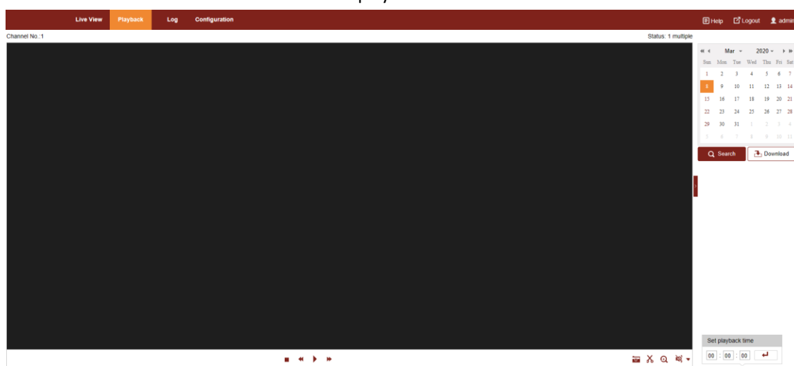
Figure 2-16 Playback Interface
