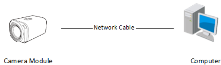
Figure 2-1 Connecting Directly
