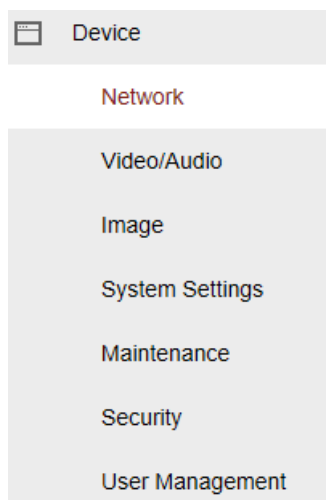
Figure 3-3 Device Setting
