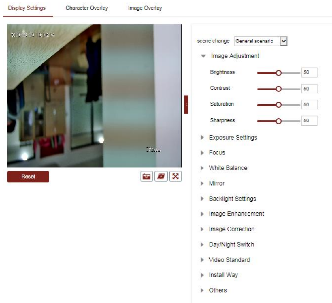
Figure 3-15 Display Setting
