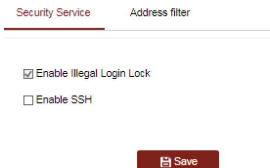
Figure 3-29 Security Service
