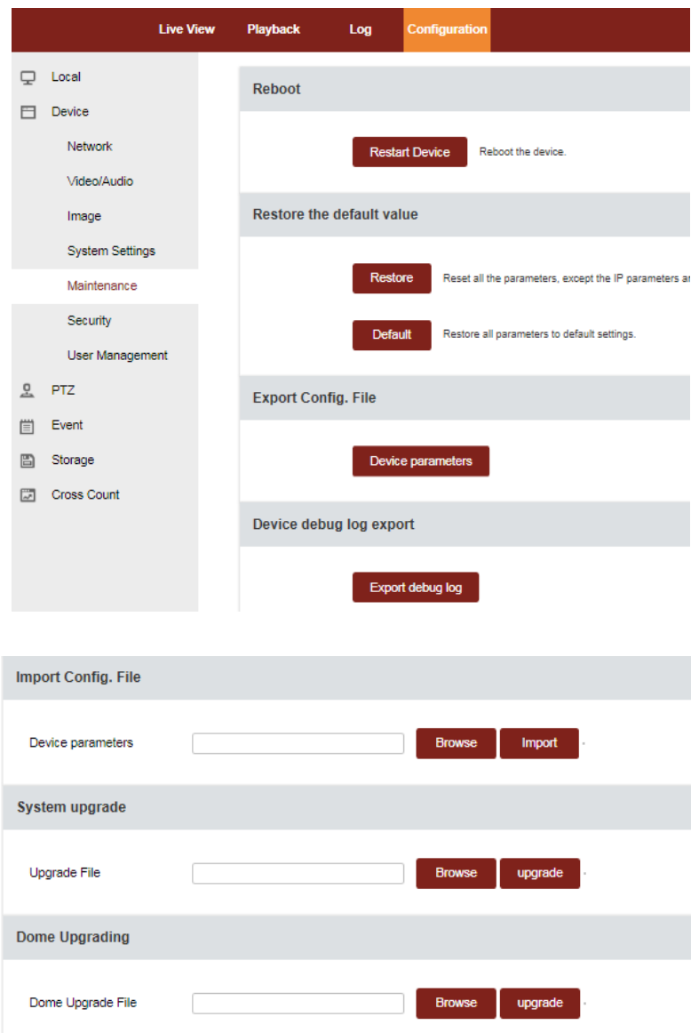
Figure 3-28 system maintain
