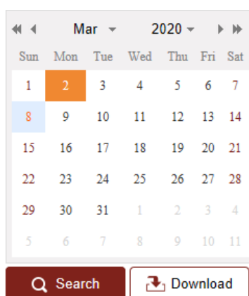
Figure 2-17 Search Video
