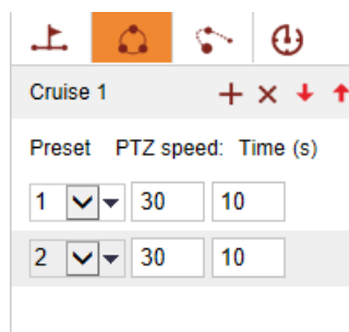
Figure 2-11 Adding Presets
