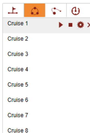
Figure 2-10
