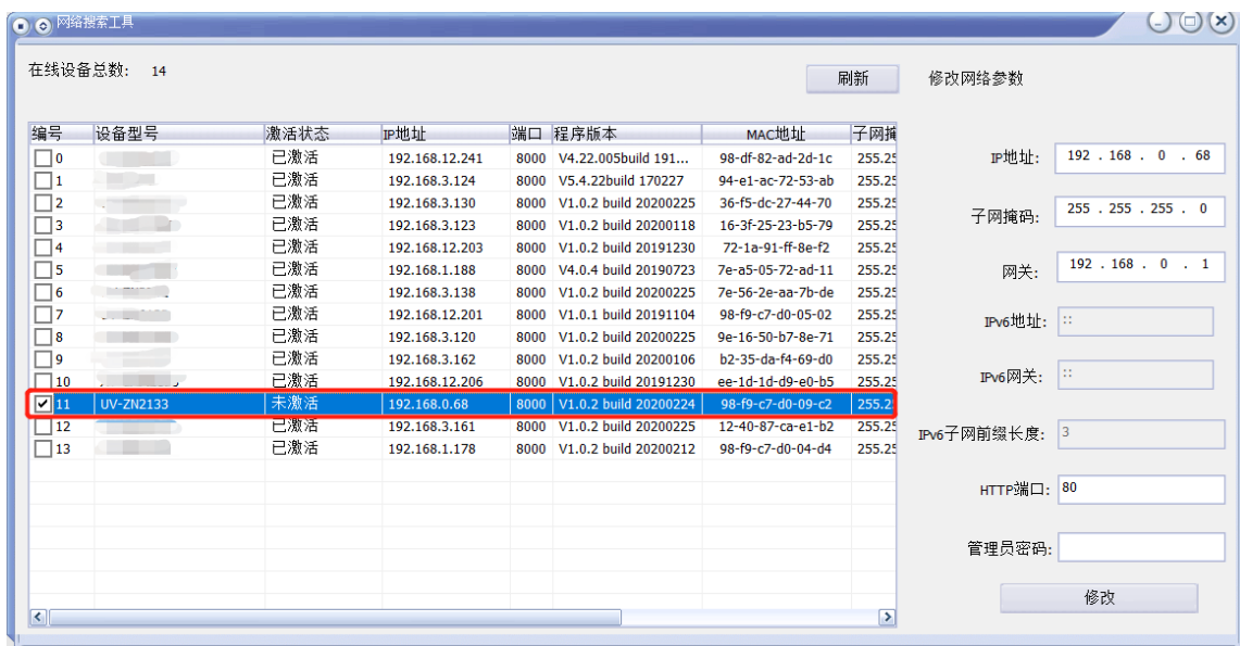
Figure 2-4 Device Active
