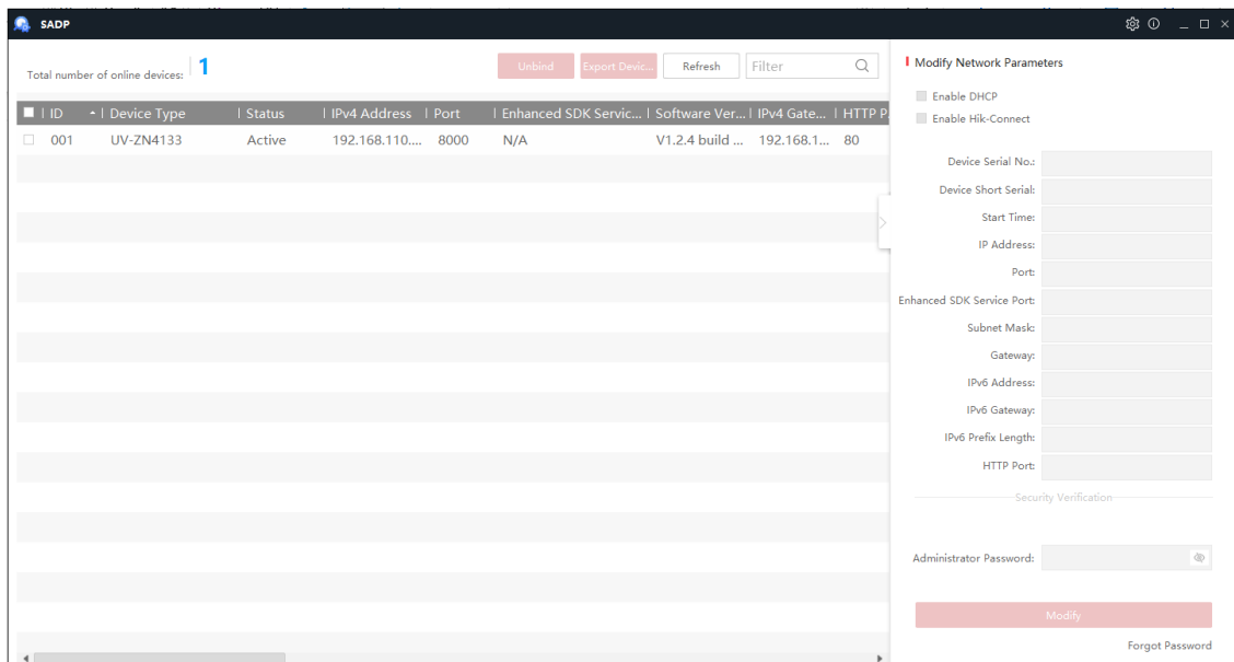
Figure 2-3 SADP Interface
