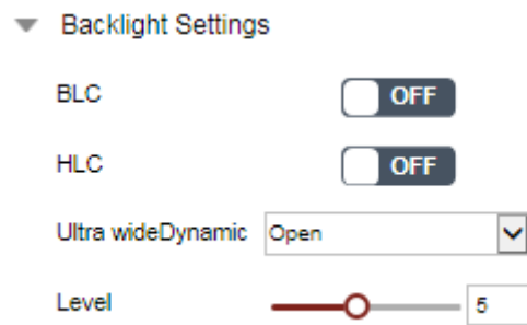
Figure 3-18 WDR
